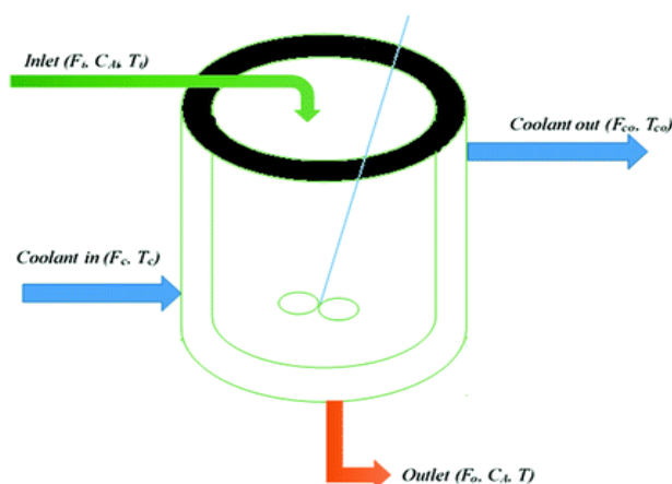
FIGURE 1. CSTR [10]
