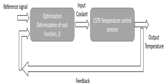
FIGURE 2. NN CONTROLLER
