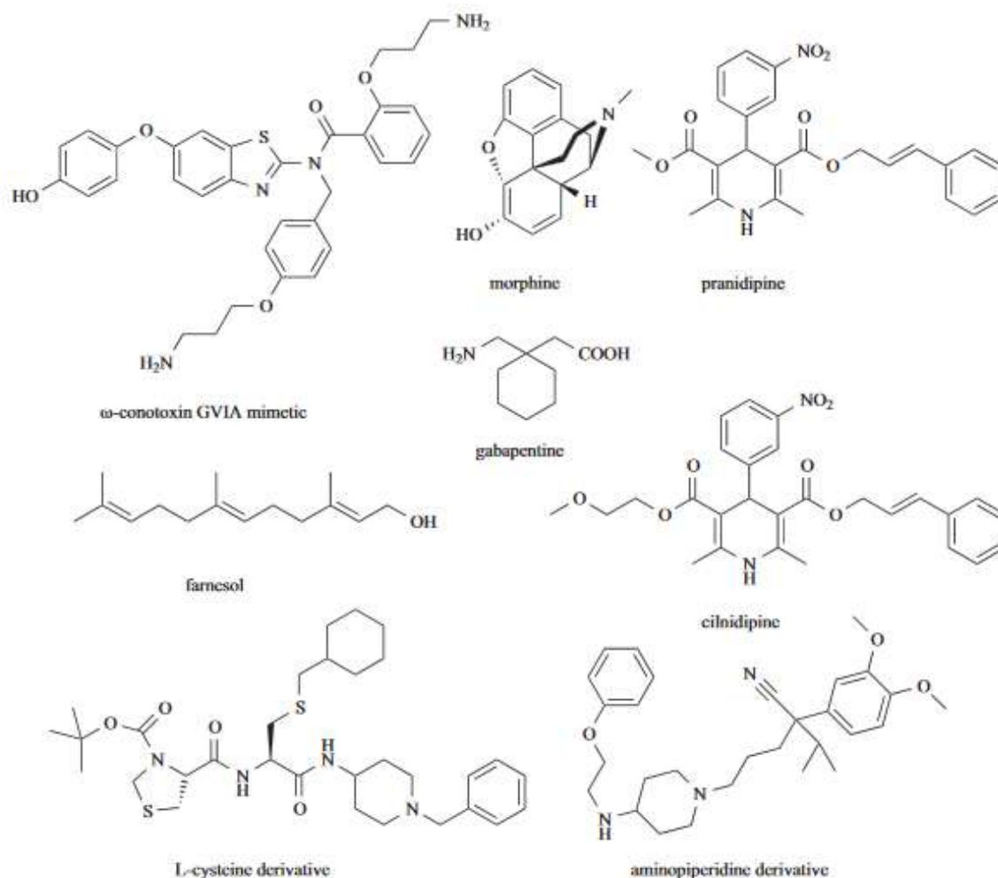
Fig. (6). Structures of some important small organic Ca v 2.2 channel blockers
