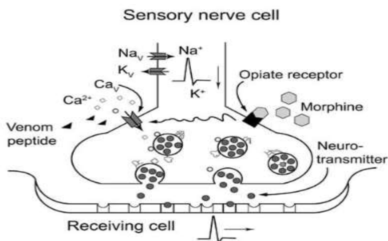
Fig. (2). Schematic figure of the presynaptic nerve terminal. Calcium influx through a Ca v 2.2 channel causes neurotransmitter release and propagation of the pain message. The propagation of the action potential and thereby the influx of calcium can be blocked by venom (e.g. Ziconotide or AM336). Activation of the opioid receptor leads to inhibition of the N-type Cav channel via G-protein coupled receptor by changing channel gating and by altering ion permeation (Adapted from Schroeder and Lewis).
