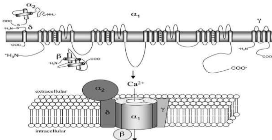
Fig. (1). Structure of VGCCs. The pore-forming 1 subunits is encoded by a single gene, and is composed of four domain, I-IV. Each do-main consists of six transmembrane helices (S1-6), with S4 serving as the voltage sensor, and the re-entrant P-loop between S5-S6 lining the pore. VGCCs associate with ancillary subunits in vivo . The \alpha_2/\delta subunit is encoded by a single gene which undergoes post-translational cleavage and rejoining by disulfide bonds to form membrane spanning \delta - and extracellular \alpha_2 -subunits. \beta -Subunits interact with the I-II linker of the channel. \gamma -Subunits also interact with the channel.
