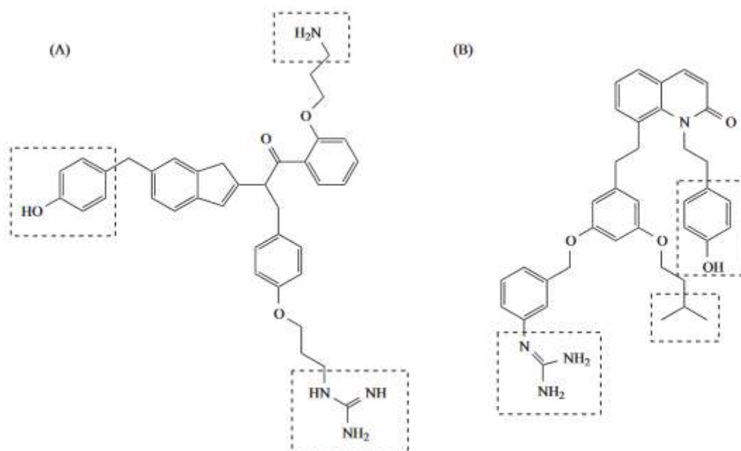
Fig. (7). Small organic \text{Ca}_v2.2 inhibitors develop using rational design. (A) Type-III mimetic. Dashed boxes indicate the three functional groups included to mimic the active residues Lys2, Tyr13 and Arg17 derived from GVIA. (B) Dendroid approach. Dashed boxes represent functional moieties included from SAR on MVIIA, Arg10, Leu11 and Tyr13. Appropriate references are found in the main text.
