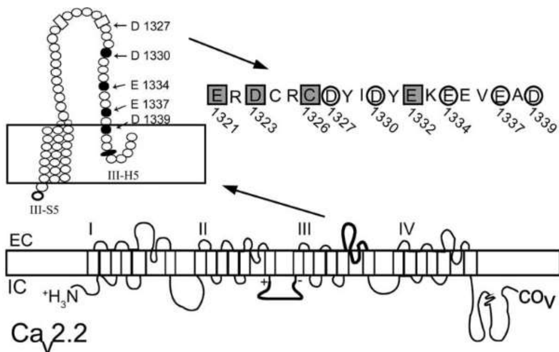
Fig. (5). Potential \omega -conotoxin binding interactions with \text{Ca}_v2.2 channel. Proposed topology of the N-type VGCC \alpha_{1B} subunit indicating the putative EF-hand motif (thick line, top) and the intracellular loop between domain II-III identified to cause change in GVIA and MVIIA binding to the channel (thick line bottom). Amino acids previously identified as important for GVIA block of the N-type VGCC (black circles) and proposed EF-hand motif (grey squares). Amino acid sequence of the \text{Ca}_v2.2 ( \alpha_{1B} ) domain III S5-H5 region indicated including Gly1326 (top right).
