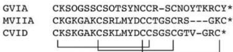
Fig. (3). Sequences and disulfide arrangement for \omega -conotoxins GVIA, MVIIA and CVID
