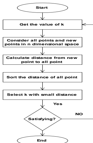
Fig.3. Flow graph of KNN algorithm
