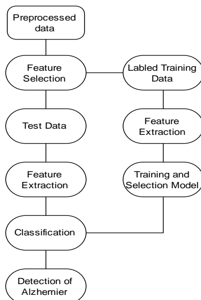
Fig 2: Flow graph of Gradient Boosting Classifier
