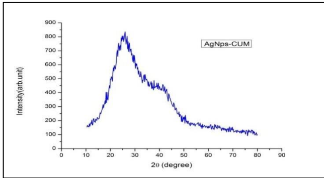
Figure 4 Shows X-ray Diffraction of Silver Nanoparticles with curcumin
