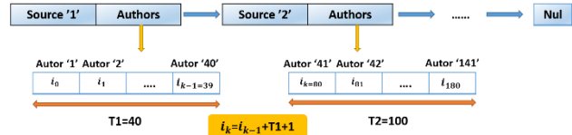
Figure 3. Calculation of authors indices
