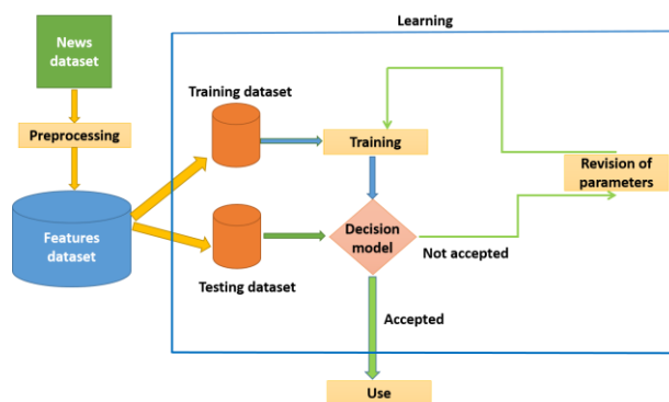
Figure 1. The proposed fake news detection system architecture's
