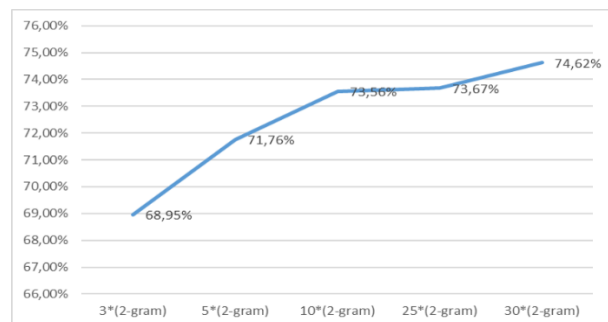
Figure 7. Evolution of the rate according to the k * (2-grams)
