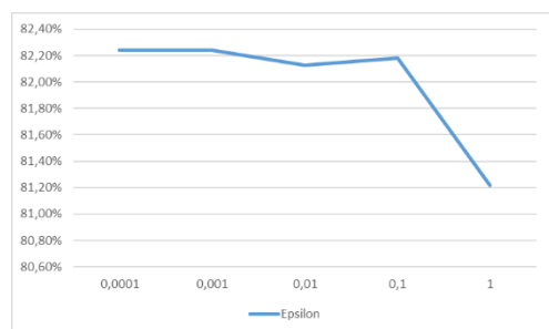
Figure 11. Evolution of the accuracy rate according to \epsilon
